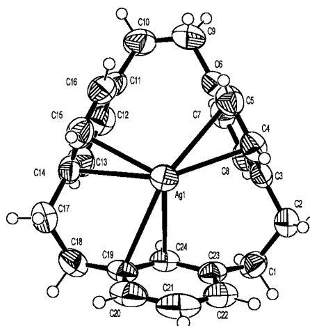
Fig. 6 ORTEP[38] plot with labeling scheme for [2.2.2] m,p,p -cyclophane-Ag-triflate ( 16 ). The thermal ellipsoids are shown at 50% probability level. The coordinated triflate anion has been omitted for clarity.
