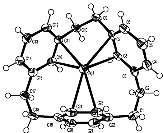
Fig. 5 ORTEP [38] plot with labeling scheme for [2.2.2] m,p,p -cyclophane-Ag-triflate ( 15 ). The thermal ellipsoids are shown at 50% probability level. The coordinated triflate anion has been omitted for clarity.
